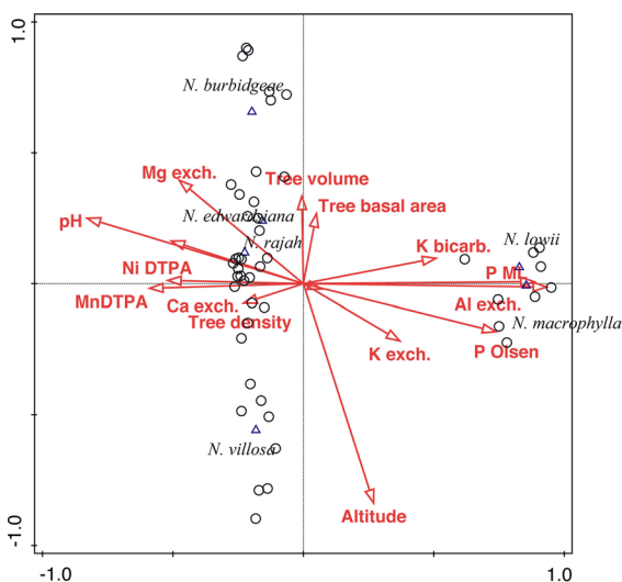
Fig. 7 CCA of soil and environmental variables in relation to Nepenthes -species. ML-3 Mehlich-3 extractable P, Olsen \text{NaHCO}_3 -extractable P, DTPA DTPA-extractable metals, exch. cations exchangeable with silver-thioarea
